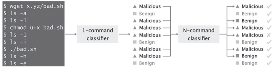
FIGURE 8. THE 1-COMMAND CLASSIFIER IS USED AS A FILTER AND ONLY COMMANDS CLASSIFIED AS MALICIOUS BY THE 1-COMMAND CLASSIFIER ARE PROVIDED TO THE 4-COMMAND CLASSIFIER. THUS, THE 4-COMMAND CLASSIFIER IS PRESENTED WITH A SEQUENCE OF COMMANDS THAT IS AN APPROXIMATION OF THE ORIGINAL MALICIOUS SEQUENCE.
