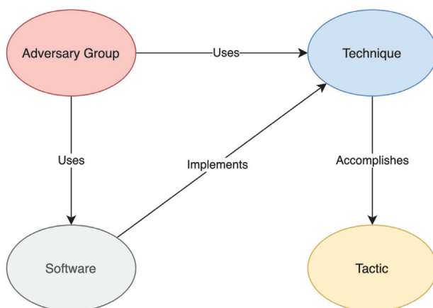
FIGURE 4: ATT&CK MODEL RELATIONSHIPS – REDESIGNED FROM [5]
